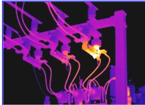
Bad Connection at Switch Shows as Thermal Anomaly
