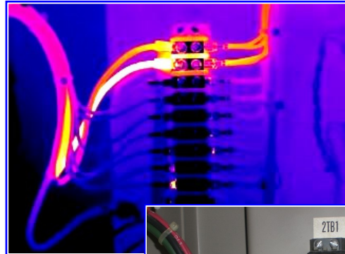
Bad Connection at Terminal Strip
